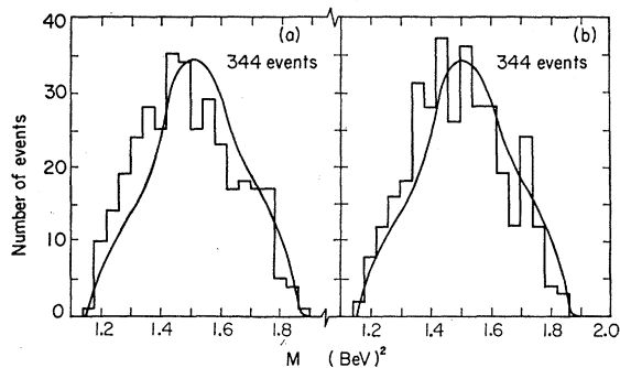
FIG. 7. Histograms of the distribution of the effective-mass squared for (a) all the pion-nucleon pairs, and (b) all the pion-antinucleon pairs. The solid curve is the same resonance-model prediction shown in Fig. 6.
