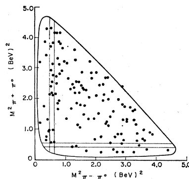
FIG. 15. An effective-mass-squared scatter diagram for the 131 events in the three-pion annihilation sample. The narrow bands indicate the position of the charged \rho meson. The neutral \rho would show up in a band near the upper right-hand edge of the envelope. However, this band is spread out considerably due to the spread in the beam momenta. The envelope corresponds to the kinematic limit for 1.61-BeV/c antiprotons.
