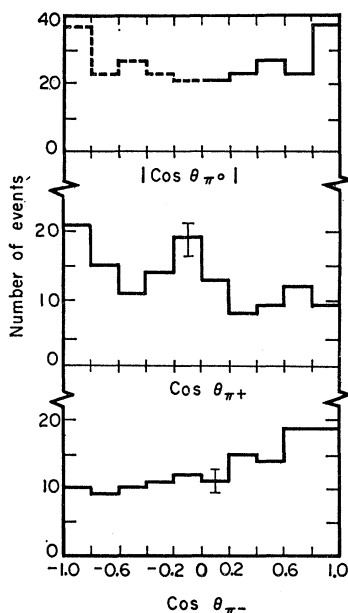
FIG. 17. Histograms of the c.m. angular distribution for the pions in the three-pion annihilation sample. The \pi^0 distribution has been folded around 90^\circ .
