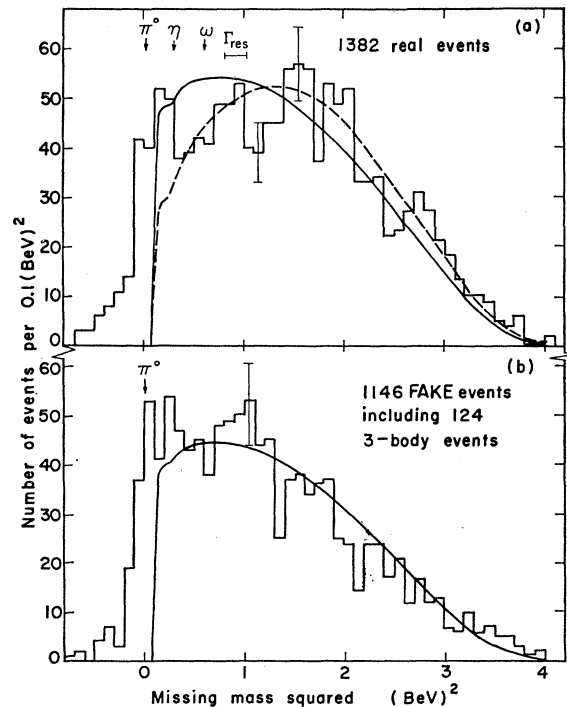
FIG. 8. A histogram of the distribution of the square of the missing mass calculated for (a) the real events in the pion-annihilation sample and (b) the FAKE events. The solid curve is the prediction based on a statistical model with \Omega=5 . The dashed curve represents an empirical model discussed in the text.
