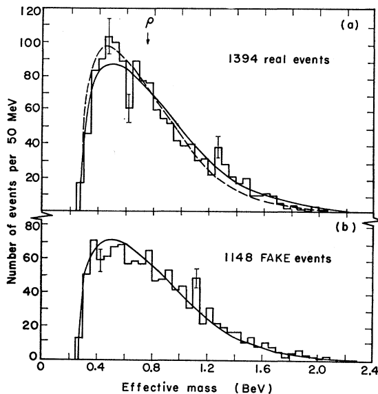
FIG. 10. A histogram of the distribution of the effective mass for the \pi^+\pi^- pair for (a) the events in the pion-annihilation sample and (b) the FAKE events. The solid and dashed curves are predictions of the same statistical model and empirical model used in Fig. 8 and Fig. 9.
