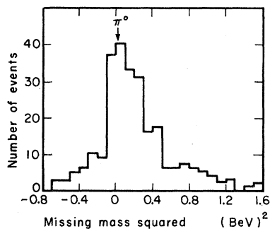
FIG. 13. Histogram of the square of the missing mass for those events in the pion-annihilation sample having \chi^2 < 5 for the three-pion interpretation.
