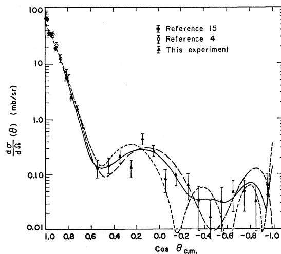
FIG. 2. The differential cross section for elastic scattering of antiprotons of 1.61 BeV/c. The data for \cos\theta > 0.8 are previously measured cross-section values, and the data for \cos\theta < 0.8 are the data from this experiment. The curves represent the best optical-model fit (dotted curve), the 6-parameter solution (dashed curve), and the best 12-parameter solution (solid curve).
