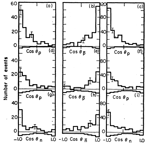
FIG. 4. The angular distributions of the nucleons and anti-nucleons in the inelastic-scattering events. Figures (a), (b), and (c) are for the \bar{p}p\pi^0 reaction, and the others are for the \bar{p}n\pi^+ and p\bar{n}\pi^- reactions. Figures (c), (f), and (i) are the appropriate sums of the two figures to the left of each. For each graph, estimates of the background events have been made; the data are plotted in such a way that the background events are plotted negatively; and the remaining events, which are the estimated number of genuine events, are plotted positively.
