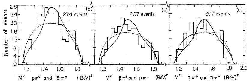
FIG. 6. Histograms of the distributions of the pion-nucleon effective-mass squared for (a) the p\pi^0 and \bar{p}\pi^0 in the \bar{p}p\pi^0 reaction, (b) the \bar{p}\pi^+ and p\pi^- , and (c) the \bar{n}\pi^+ and n\pi^- in the other two reactions. The data are compared with a phase-space estimate (dashed curve), and with the prediction based on the production of either the pion nucleon pair or the pion-antinucleon pair in the (\frac{3}{2}-\frac{3}{2}) resonance (solid curve). All curves are normalized to the data.
