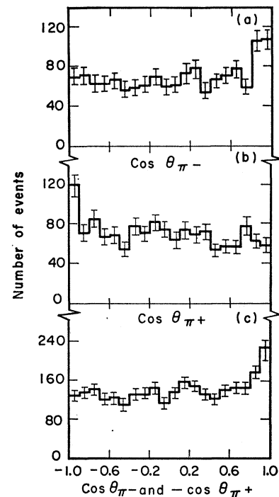
FIG. 11. A histogram of the c.m. angular distribution of (a) the negative pion, (b) the positive pion, and (c) both pions for the events in the pion-annihilation sample.
