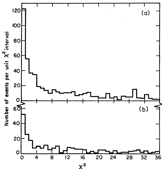
FIG. 12. Histograms of the \chi^2 distributions for the \pi^+\pi^-\pi^0 interpretation for (a) the real events and (b) a sample of 424 simulated four-pion annihilations.
