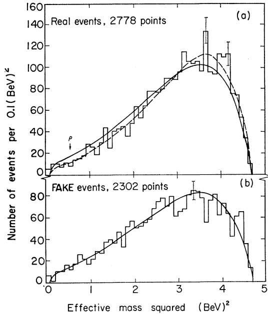
FIG. 9. A combined histogram of the square of the effective mass of everything except one of the charged particles for (a) the real events in the pion-annihilation sample and (b) the FAKE events. The solid and dashed curves are predictions of the same statistical model and empirical model used in Fig. 8.
