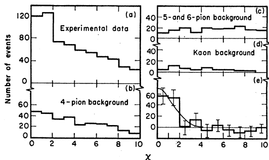
FIG. 14. Histograms of the distributions in \chi (the square root of \chi^2 ) for (a) the real events, (b) the estimated background from four-pion annihilations, (c) the estimated background from five- and six-pion annihilations, (d) the estimated background from annihilations with k mesons, and (e) the difference between the real data and the estimated background.
