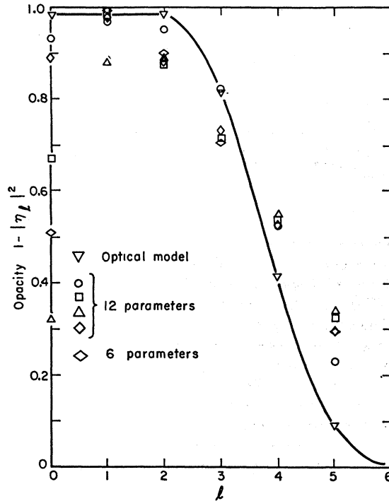
FIG. 3. A plot of the opacity ( 1 - |\eta_l|^2 ) of the proton-antiproton system for various cases. The smooth curve represents the best four-parameter optical-model fit to the data. The points represent the indicated solutions.
