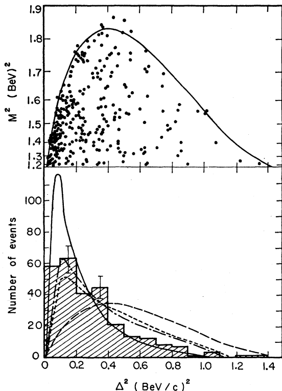
FIG. 5. A scatter diagram in the M^2, \Delta^2 plane, where \Delta^2 is the invariant four-momentum transfer of the nucleon or antinucleon and M is the effective mass of the other two particles. The M^2 scale has been distorted in such a way that, according to the Chew-Low formula, any vertical strip would be populated according to \sigma(M) , the \pi p cross section. Each event has been plotted twice on this diagram. A histogram of the projection of these data on the \Delta^2 axis is compared with a phase-space prediction (dashed curve); with the prediction indicated by the Chew-Low formula (dot-dash curve); with a modified prediction, based on the Chew-Low formula, including the distribution for both of the nucleons (dotted line); and with a similar prediction based on a peripheral model with a (\Delta^2 + m_\pi^2)^{-2} dependence (solid line). All curves are normalized to the data.
