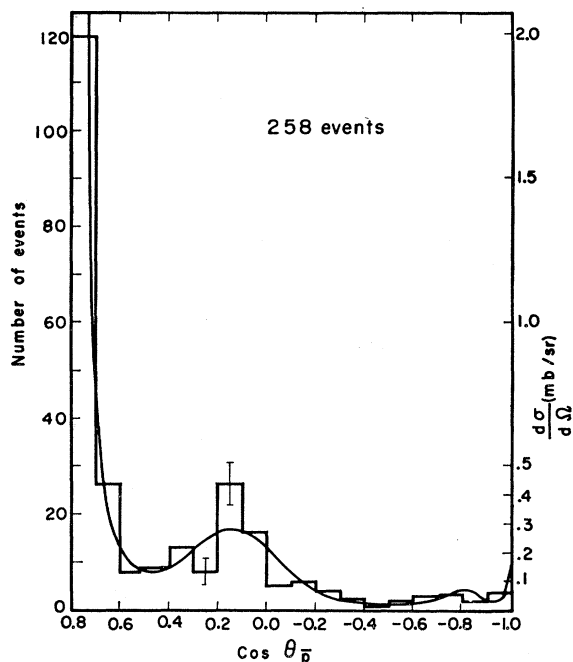
FIG. 1. A histogram of the measured differential cross section for elastic scattering of 1.61-BeV/c antiprotons for \cos\theta < 0.8 . The errors are statistical only. In addition, there is about a 6% systematic uncertainty. The curve corresponds to solution 2 in Table II.
